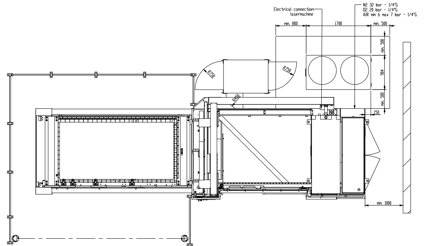
LAYOUT WITH 4 kW RESONATOR
