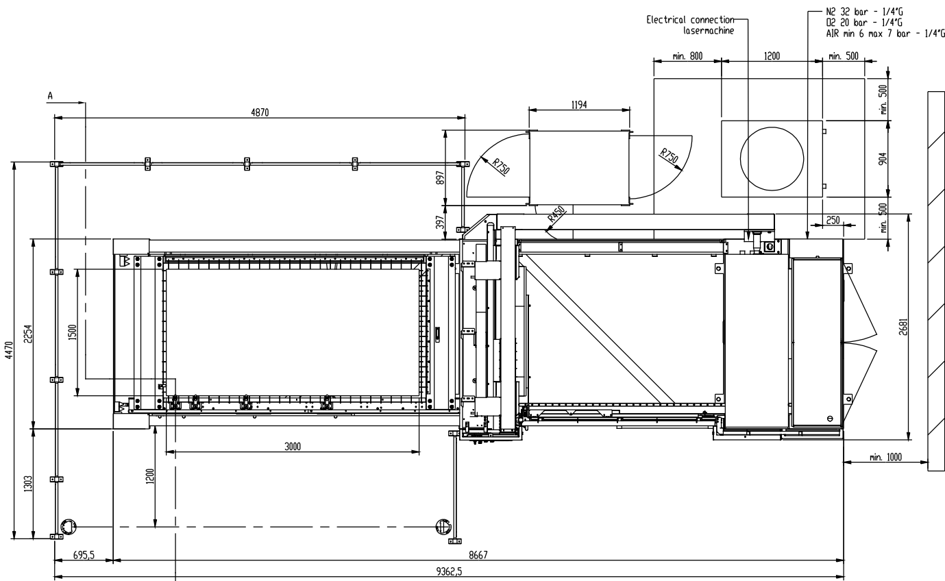
LAYOUT WITH 2,5kW RESONATOR
